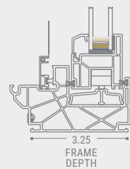
3.25 FRAME DEPTH FINLESS
